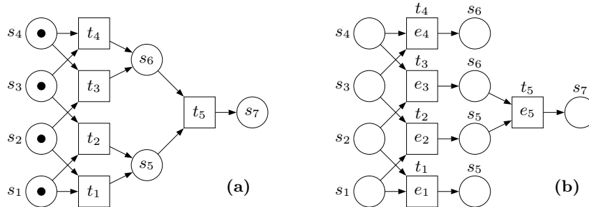
Fig. 1. A Petri net (a) and one of its branching processes (b) , which is complete according to [5], but not w.r.t. Definition 4: the configuration \{e_1, e_4\} does not preserve firings and introduces a fake deadlock. To make the prefix complete w.r.t. Definition 4, one has to add an instance of t_5 consuming the conditions produced by e_1 and e_4 .
