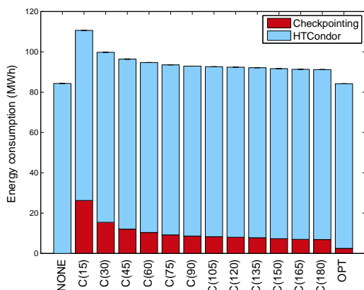
Figure 5: Energy Consumption.
