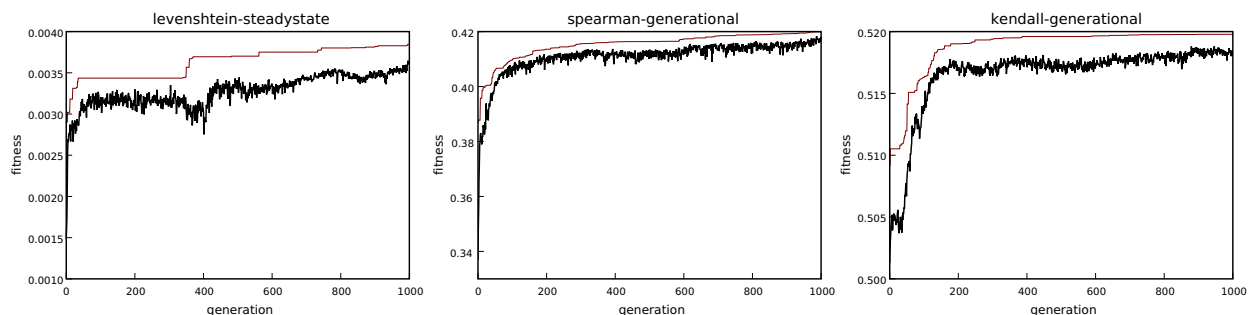
Fig. 4. Fitness throughout the generations in the first round of experiments for the best run for each fitness function. The lines show average (thick black line) and the maximum (thin red line) fitness in the population.
