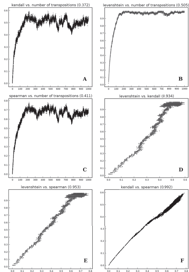
Fig. 3. Correlation between fitness and number of transpositions applied to the reference ranking (plots A–C) and direct correlation between fitness functions (plots D–F). The correlation coefficients are given in brackets.
