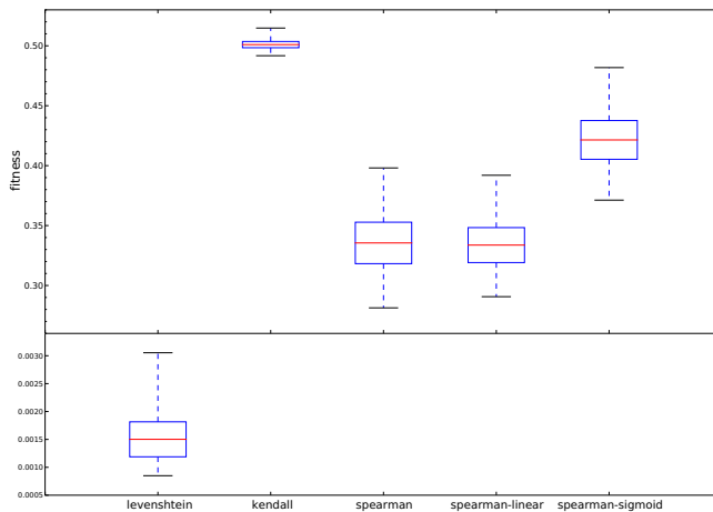
Fig. 6. Box plot of the fitness distribution achieved by a random walk for different fitness functions. Middle line is the median of the average fitness in population across all generations. Box size represents the median of the population fitness standard deviation. Top and bottom whiskers marks maximum and minimum fitness across all individuals.
