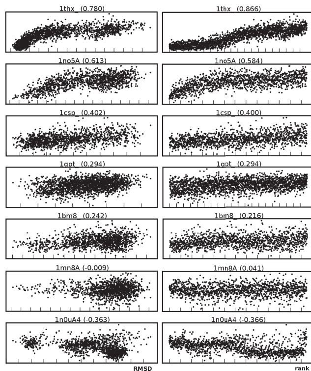
Fig. 2. Scatter plots of Rosetta original energy (vertical axis) vs. RMSD (left column) and rank (right column). Each plot represents decoys for a single protein. The correlation coefficients are given in brackets.
