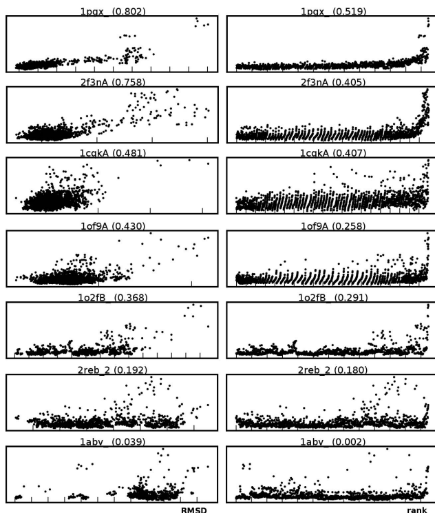
Fig. 1. Scatter plots of I-TASSER original energy (vertical axis) vs. RMSD (left column) and rank (right column). Each plot represents decoys for a single protein. The correlation coefficients are given in brackets.
