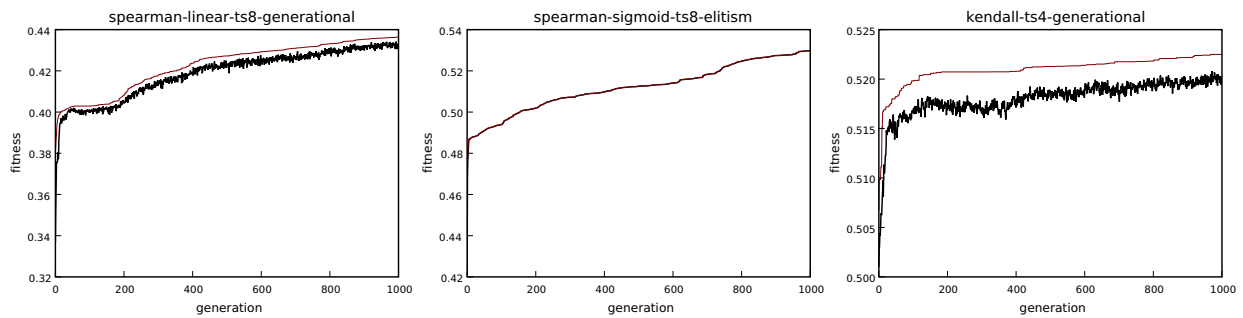
Fig. 5. Fitness throughout the generations in the second round of experiments for the best run for each fitness function. The lines show average (thick black line) and the maximum (thin red line) fitness in the population.
