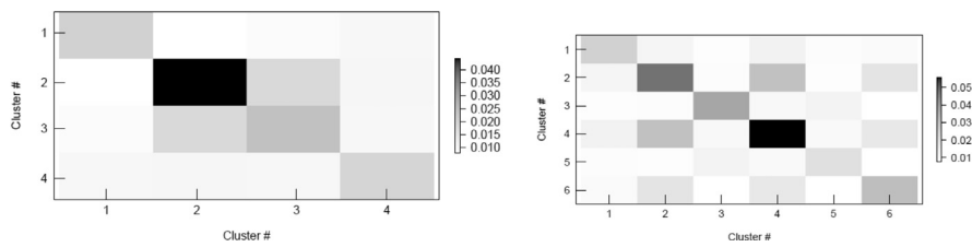
Fig. 3. Inter- and intra-similarity for 4 and 6 clusters topic models.
