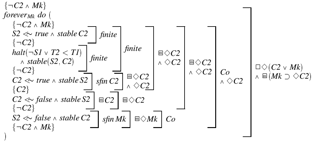
Figure 22: Proof outline for lemma (45).
