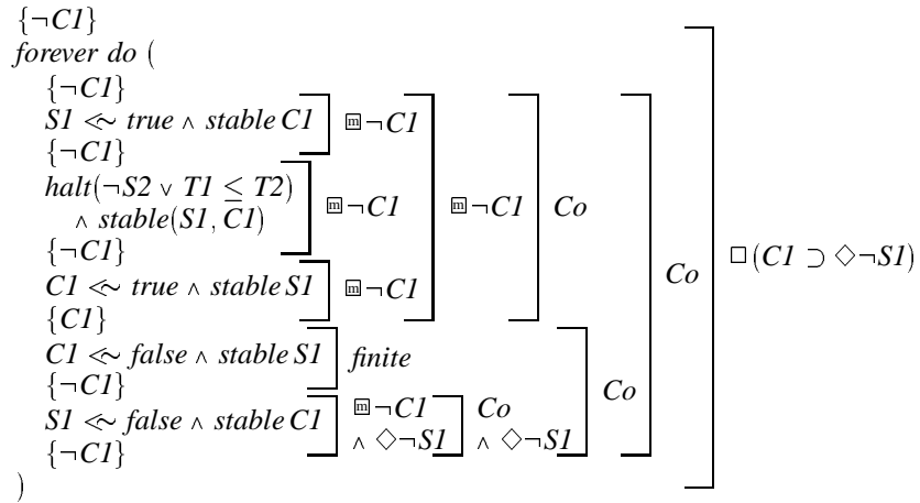
Figure 20: Proof outline for lemma (42).
