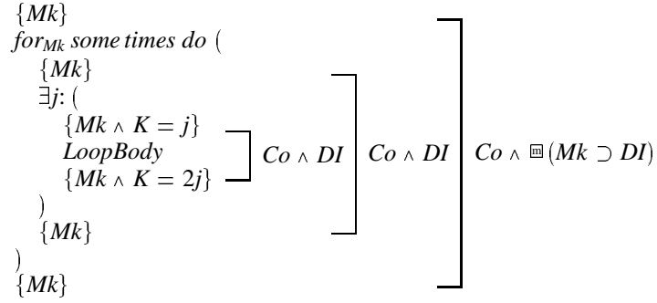
Figure 6: Proof outline for lemma (11).
