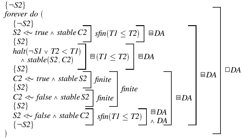
Figure 19: Proof outline for lemma (40).
