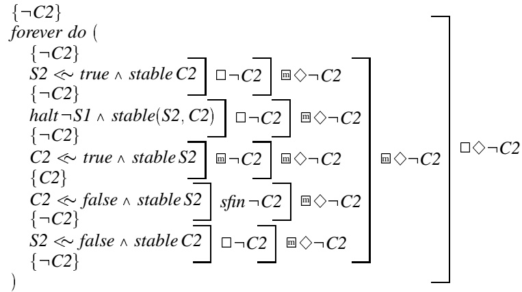
Figure 14: Proof outline for lemma (30).
